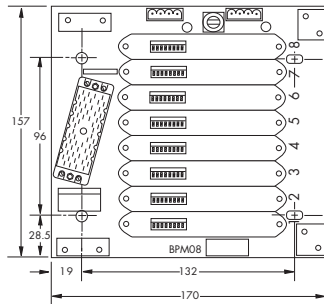
BPM08 8-way backplane (multiway connectors)
